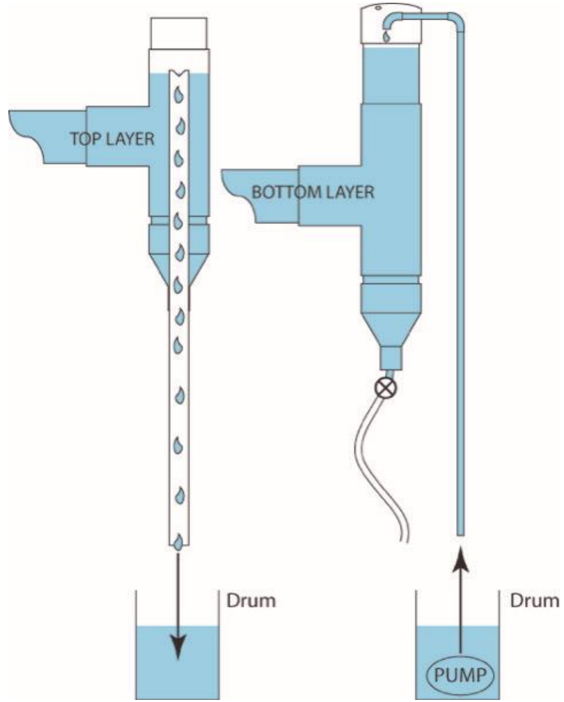
Drain and overflow design of water battery
